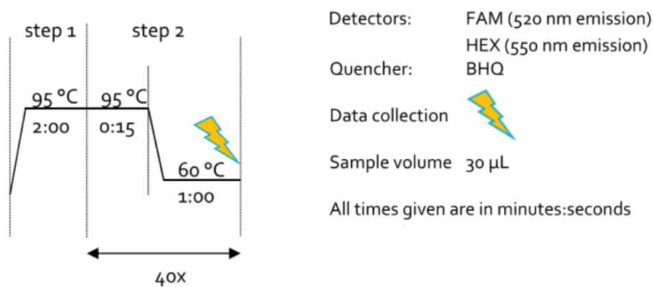
Figure 2. Temperature scheme of thermocycler.
